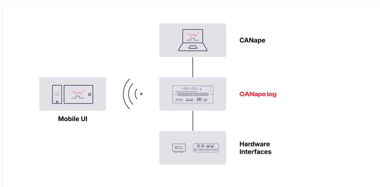
FIGURE 13: CANape log is a member of the new Vector Smart Logger family. The powerful combination of CANape and dedicated logger hardware enables time-synchronous and high-performance recording of measurement data.
