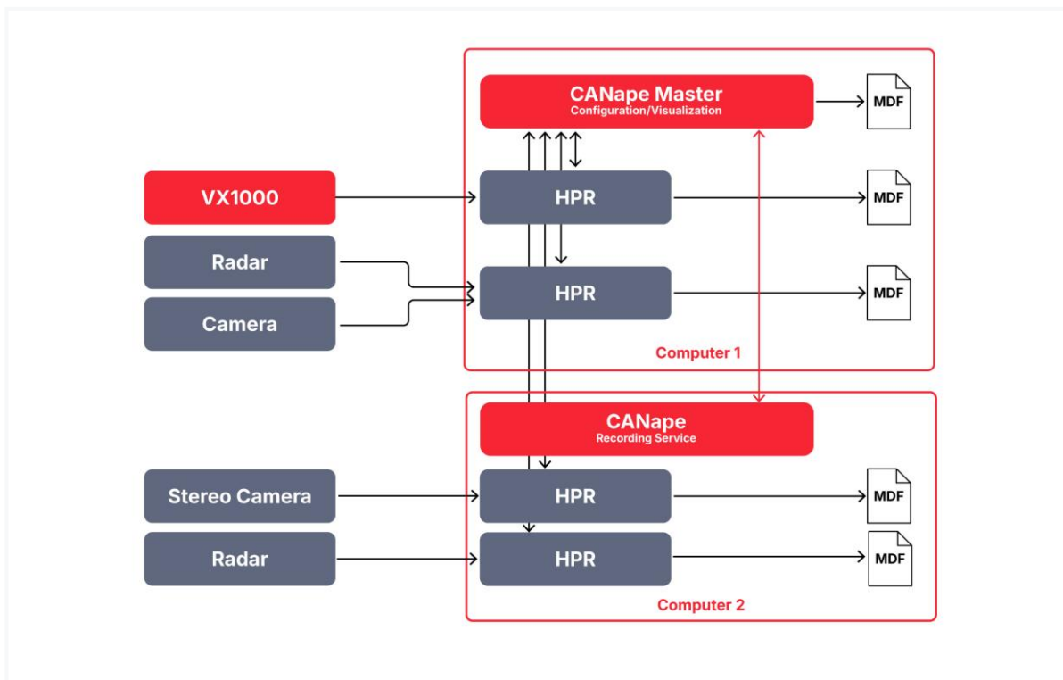
FIGURE 3: Scalable decentralized recorder solution for very large data rates in the ADAS environment
