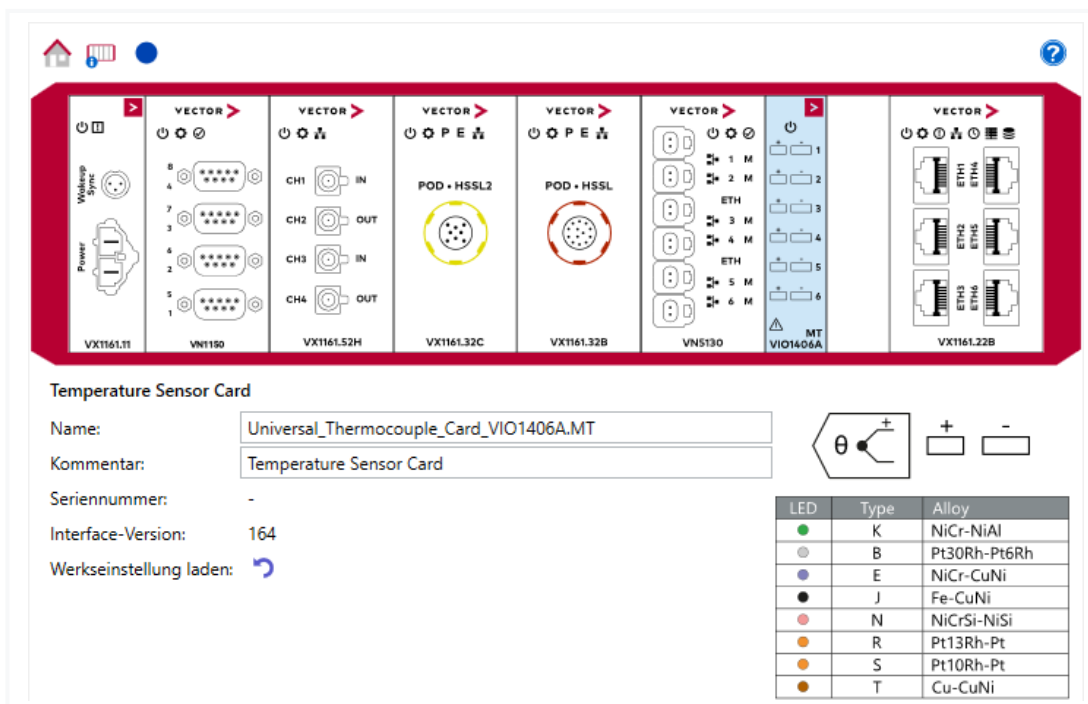
FIGURE 6: Hardware configuration dialog for VIO System in CANape. The depicted hardware is a VX1161 with network interface, streaming, POD and a VIO1406A.MT card.
