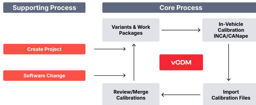
Figure 26: Overview calibration process in vCDM
