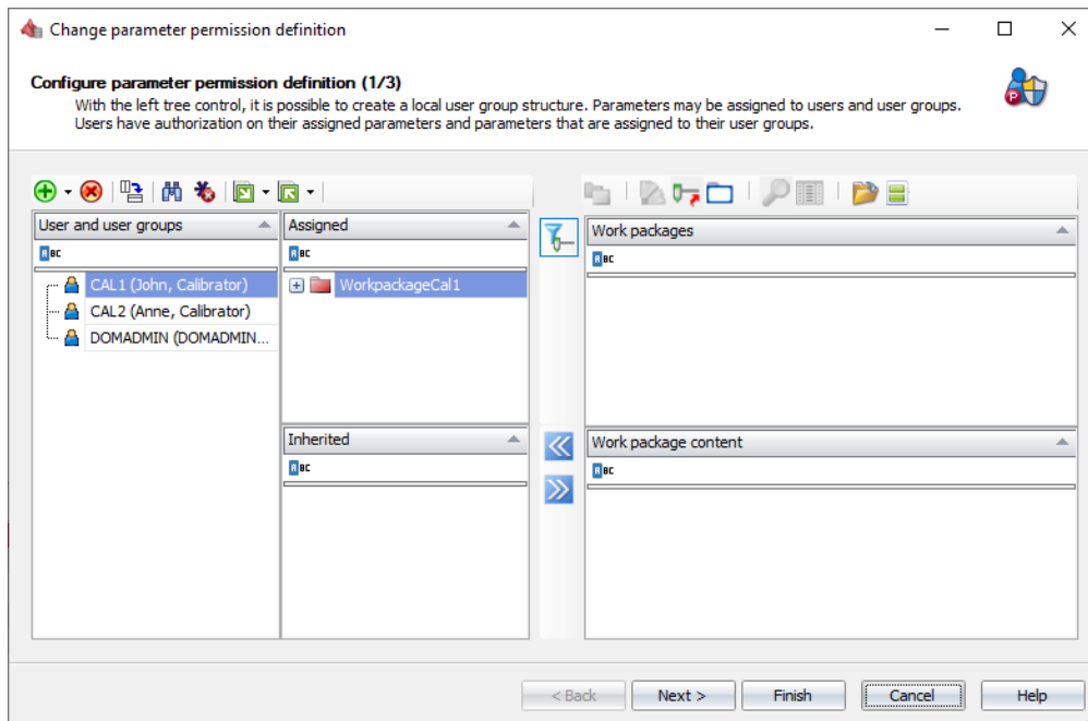
Figure 22: Parameter Permission Editor
