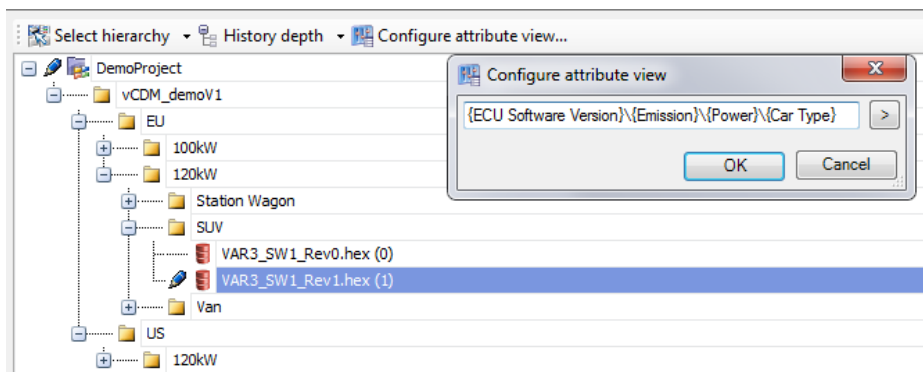
Figure 20: Data set variants grouped in folders
