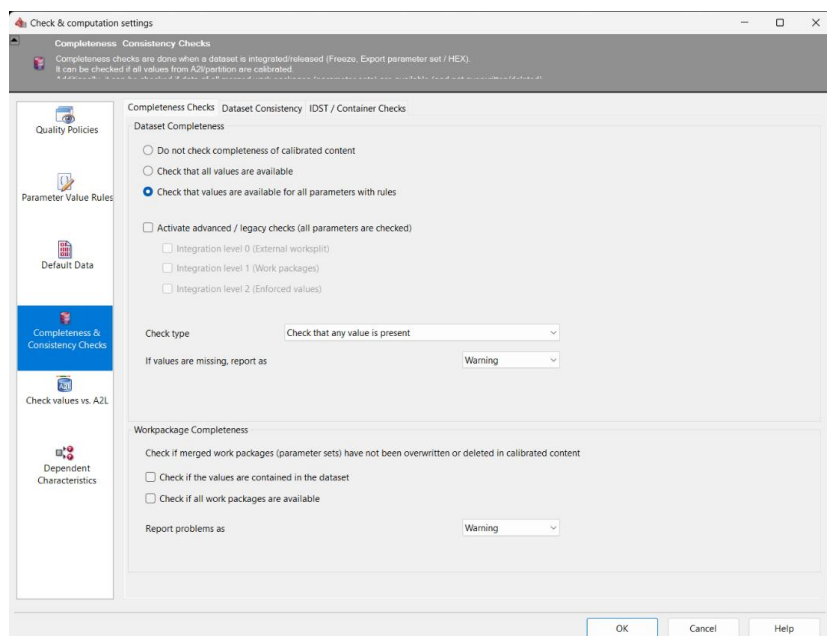
Figure 28: Setup Required Data Quality for the vCDM Validation Framework
