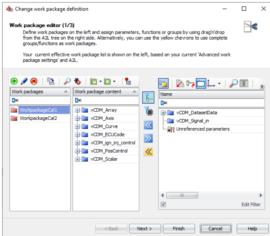
Figure 21: Work packages can be easily defined in the editor
