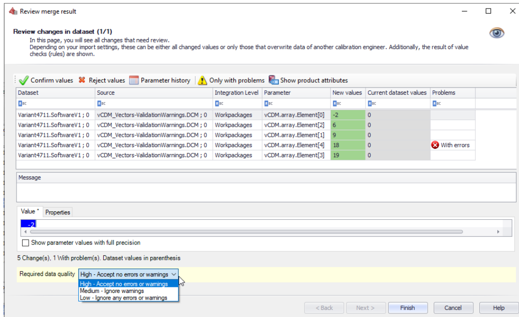
Figure 27: Approval of parameter changes
