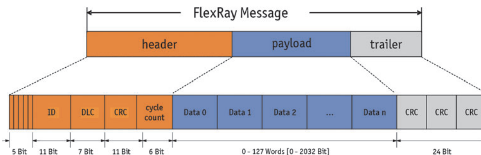
Figure 6: Structure of the FlexRay message with header, payload and trailer.
