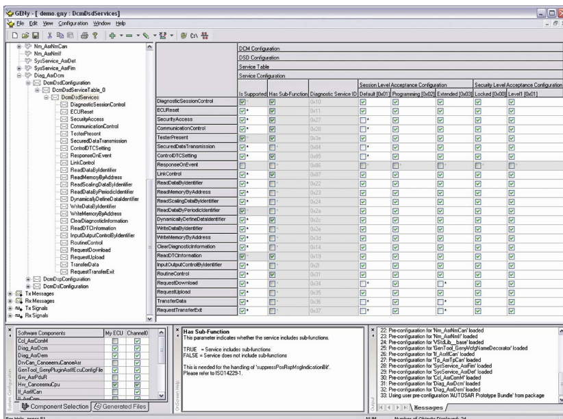
Configuring MICROSAR DIAG with GENy
