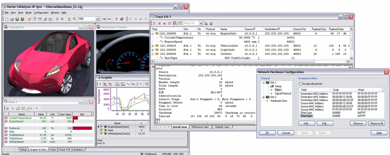
CANalyzer.IP configuration for displaying signals. The Ethernet protocol and signal decoding are analyzed in the Trace Window. Acceptance filter for reducing the number of packets.
